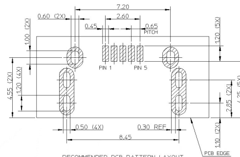
RECOMMENDED PCB PATTERN LAYOUT GENERAL TOLERANCE: ±0.05
