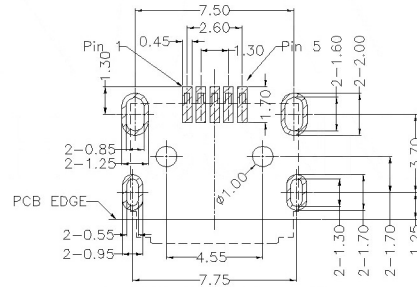
RECOMMENDED PCB LAYOUT TOP VIEW(.XX±0.05)
