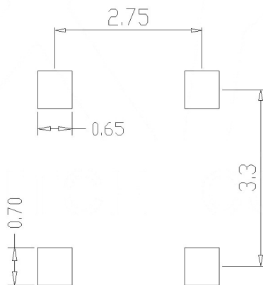
PCB.circuit prohibited area
