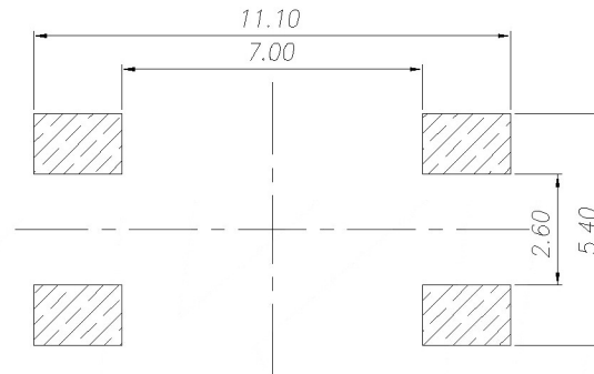
P.C.B Mounting pattern Dimension
