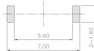
P.C.B Mounting pattern Dimension
