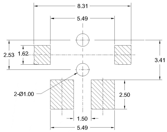
Recommended Layout
