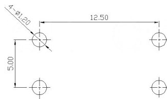
P.C.B MOUNTING PATTERN DIMENSION
