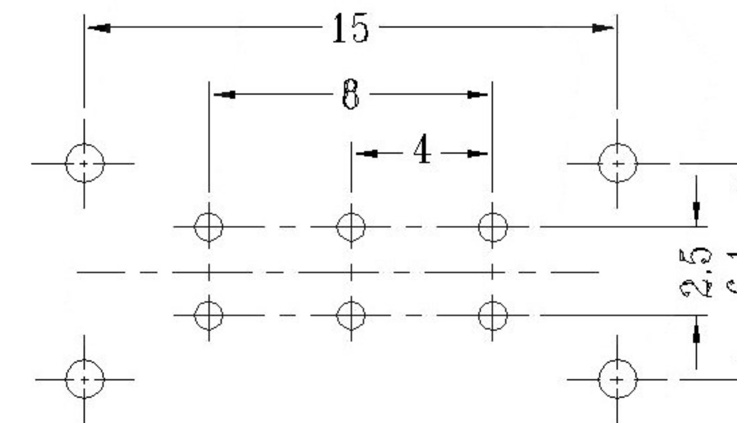
P.C.B LAYOUT BOTTOM VIEW
