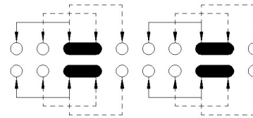
SCHMATIC (SHORTING)
