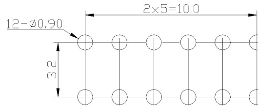
P. C. B LAYOUT
