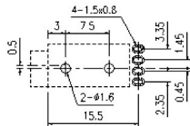
P.C.B. LAYOUT TOP VIEW
