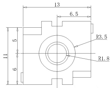
PJ-344X-1
