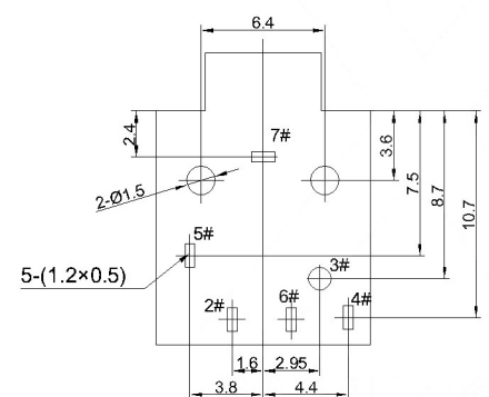
PCB Holes diagram Top View
