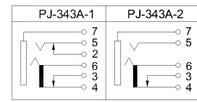
SCHEMATIC
