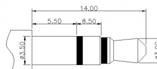
ø3.50mm 3 POLE PLUG
