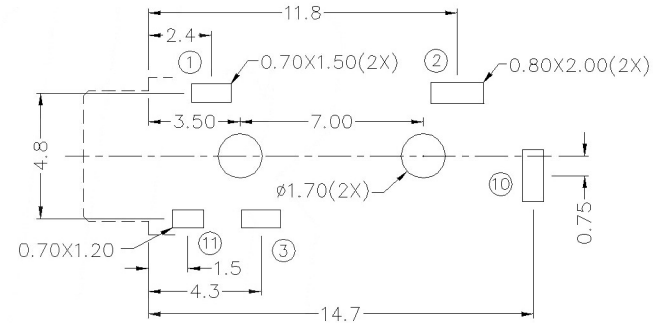
RECOMMENDED (BOTTOM VIEW)
