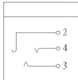
Ø3.50mm 3 POLE PLUG
