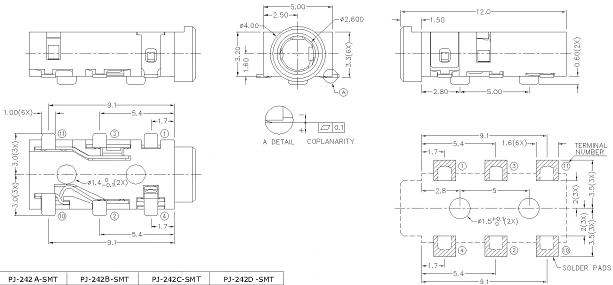
Recommended PCB Layout Top View
