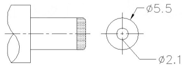
MATING PLUG Jack Insertion Depth: 9.0 mm
