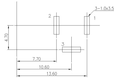
PCB LAYOUT TOP VIEW TOLERANCES:±0.05
