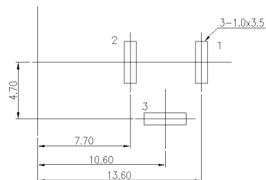
PCB LAYOUT TOP VIEW TOLERANCES: ±0.05
