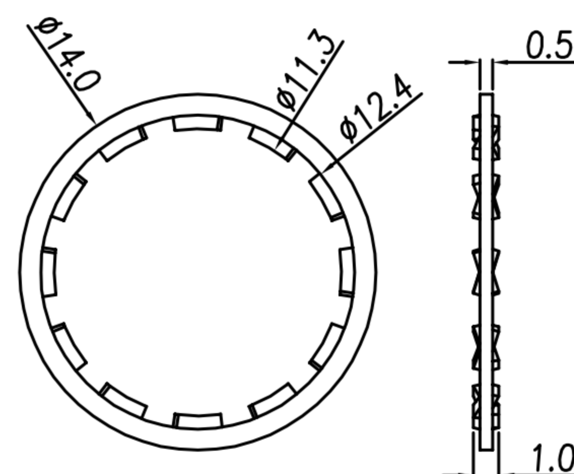
WASHER
