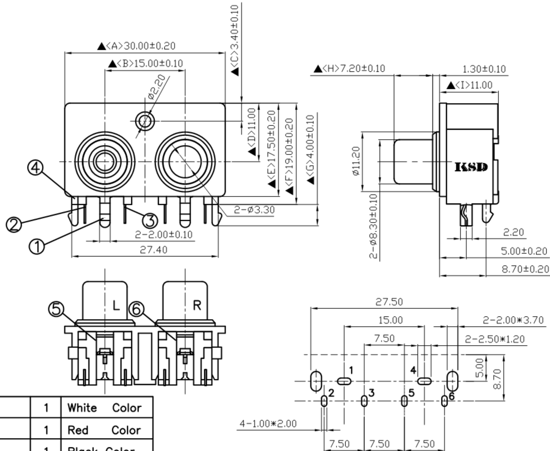
Pin Hole Layout (Jack Bottom View)
