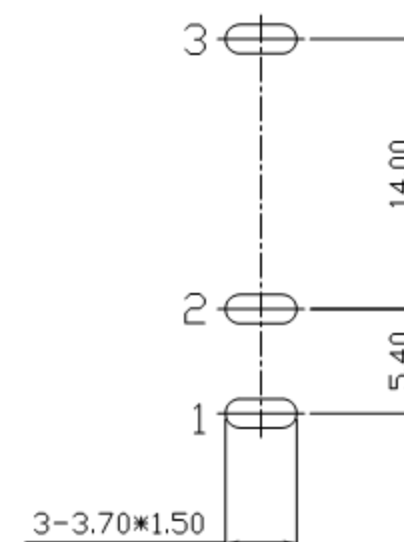
Pin Hole Layout (Jack Bottom View)
