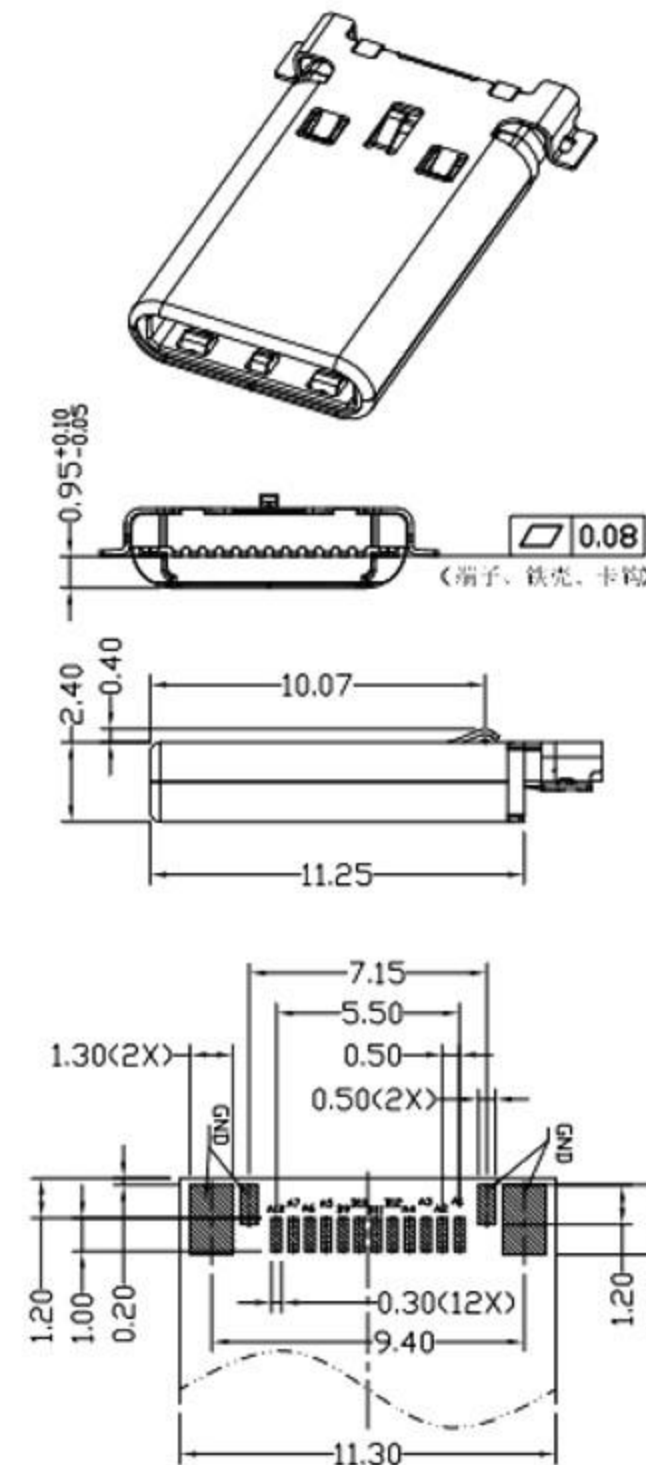
RECOMMENDED PCB LAYOUT(TOP VIEW) TOLERANCE:±0.05
