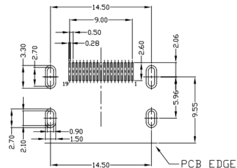
RECOMMENDED PCB LAYOUT (T=1.60mm)
