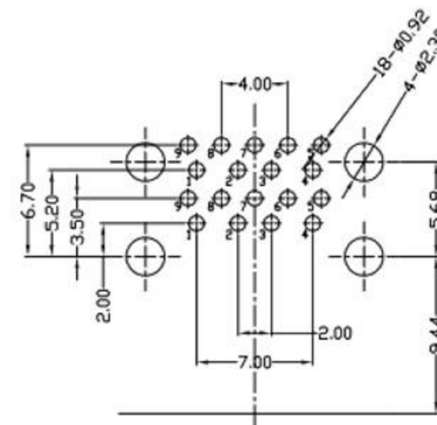
RECOMMEND PCB LAYOUT
