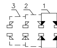
NON-SHORTING SCHEMATIC
