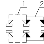
NON-SHORTING SCHEMATIC
