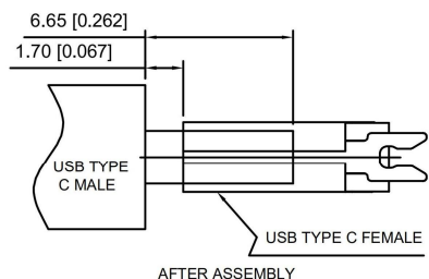
AFTER ASSEMBLY
