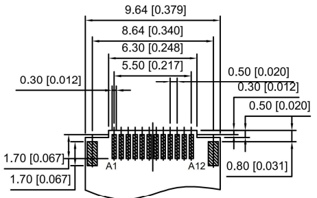
RECOMMENDED PCB LAYOUT(TOP VIEW) THICKNESS 0.80±0.05MM;DEFAULT TOLERANCE:±0.05
