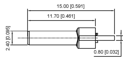
SECT B-B
