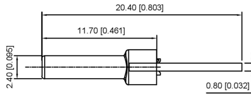
SECT B-B
