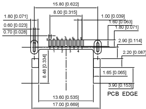
RECOMMENDED PCBA LAYOUT (TOLERANCE±0.05)
