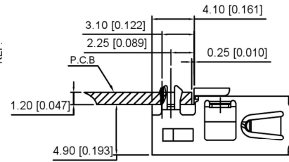
PROPOSAL DRAWING
