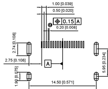
RECOMMENDED PCB LAYOUT TOL:±0.05
