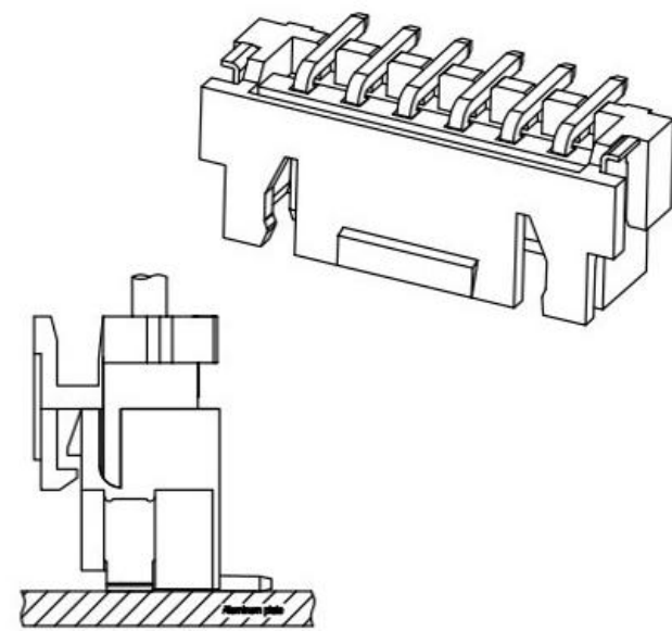
Assembly Layout
