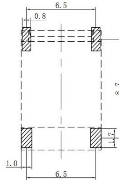
PCB BOARD LAYOUT
