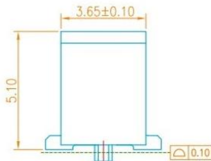
MATING HEIGHT SCALE:1.25:1
