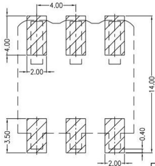
Board Layout
