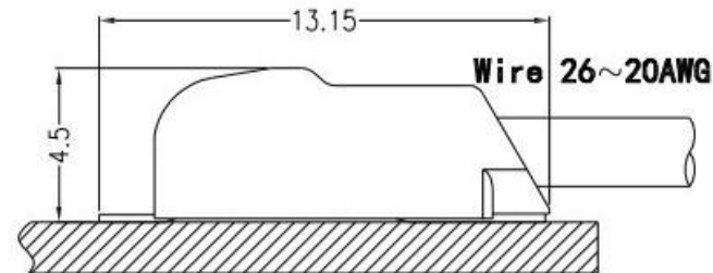
Installation drawing
