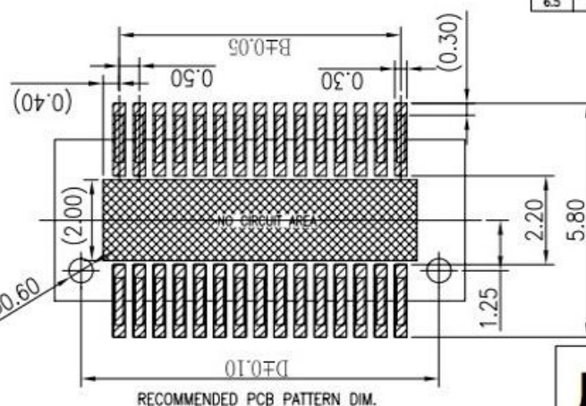
RECOMMENDED PCB PATTERN DIM.
