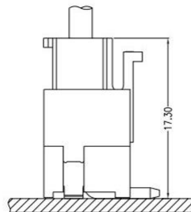
Assembly Layout
