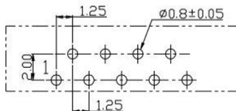
RECOMMEND PCB LAYOUT COMPONENT SIDE (FOR PD15-XX0XAW)
