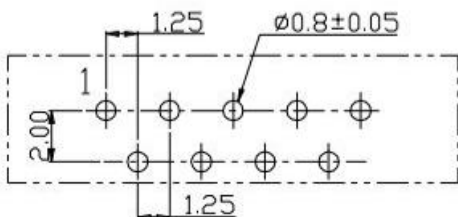
RECOMMEND PCB LAYOUT COMPONENT SIDE (FOR PD15-XX0XA)
