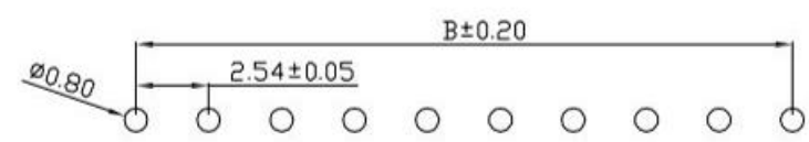
PCB LAYOUT
