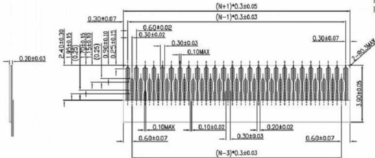
APPLY FPC RECOMMENDED DIM (THICKNESS 0.20±0.03)
