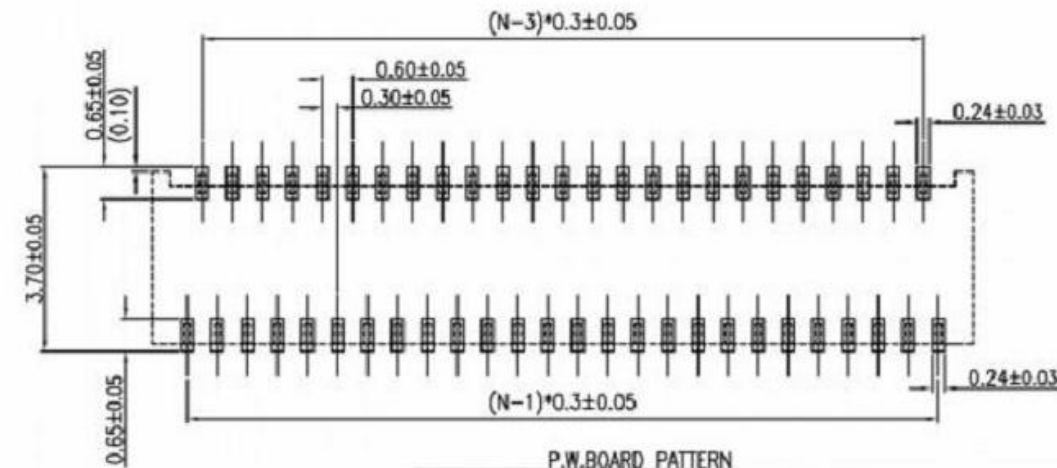
P.W. BOARD PATTERN RECOMMENDED METAL MASK THICKNESS 0.1mm
