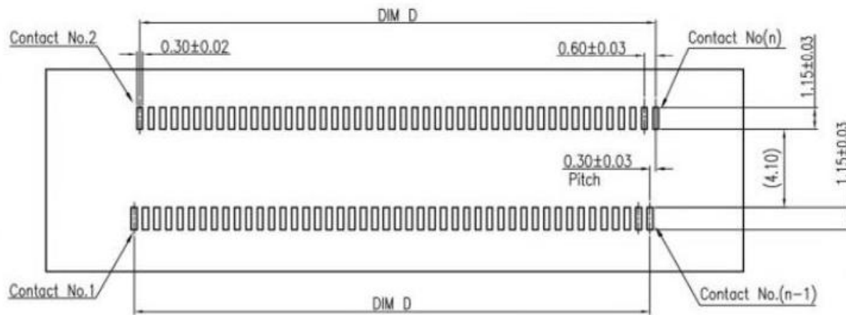
Recommended PCB and Metal Dimension (Connector Mounting Surface)
