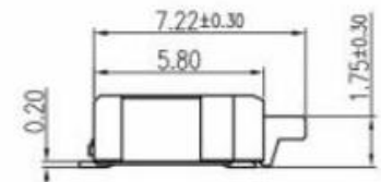
STYLE OF LOCK LEVER CLOSE
