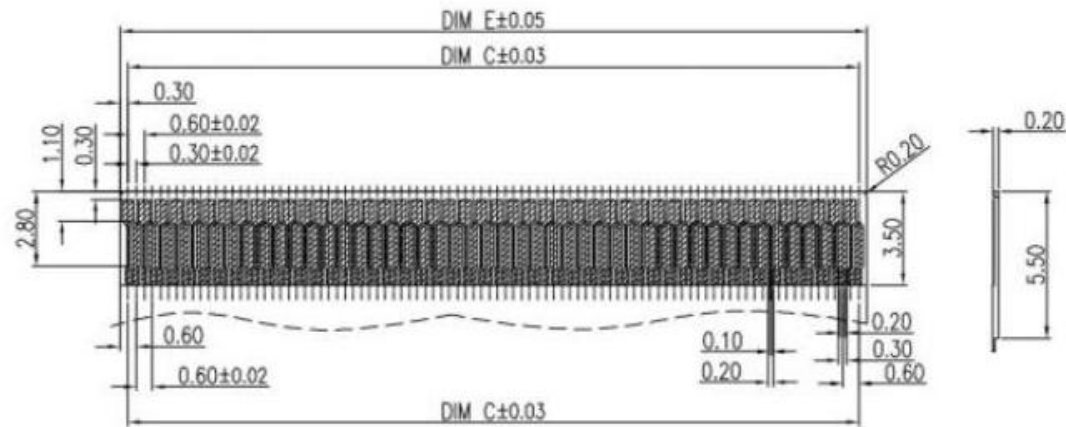
Recommended FPC/FFC Dimension
