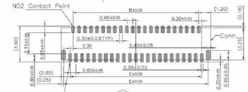
FPC/FFC Insert Direction Recommended P.C.B Layout
