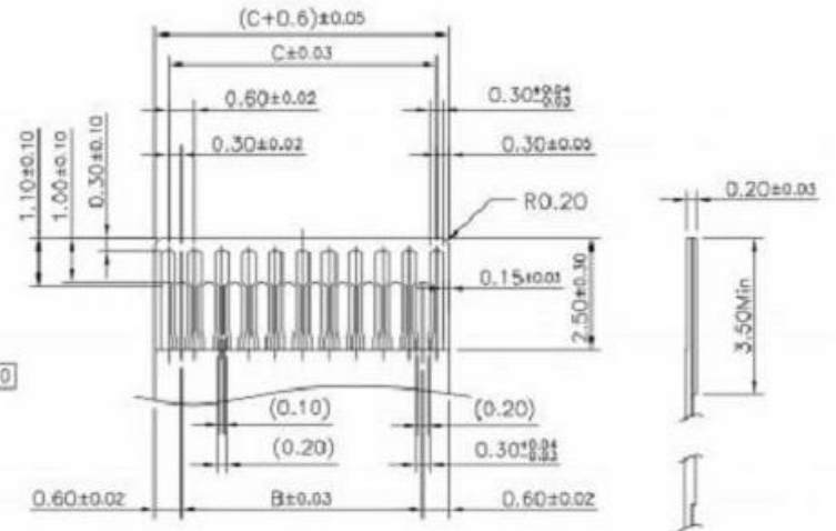
Applicable FPC
