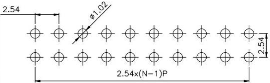
PCB LAYOUT
