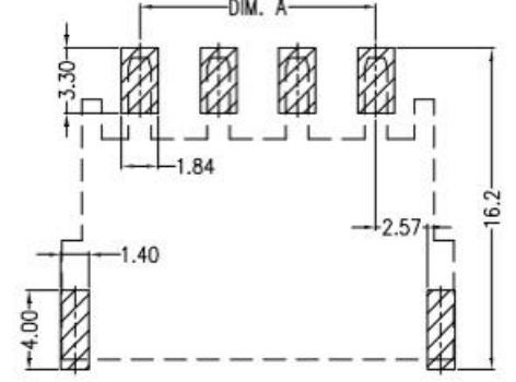
Mating PCB detail
