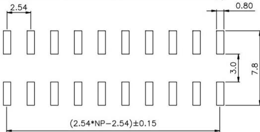
PCB LAYOUT
