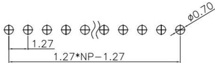
PCB LAYOUT
