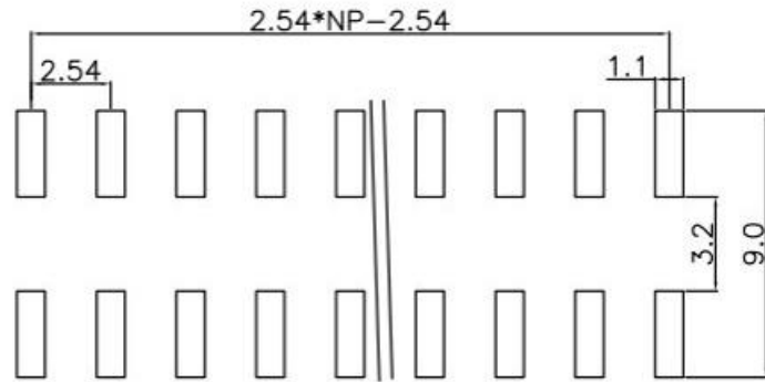
PCB LAYOUT
